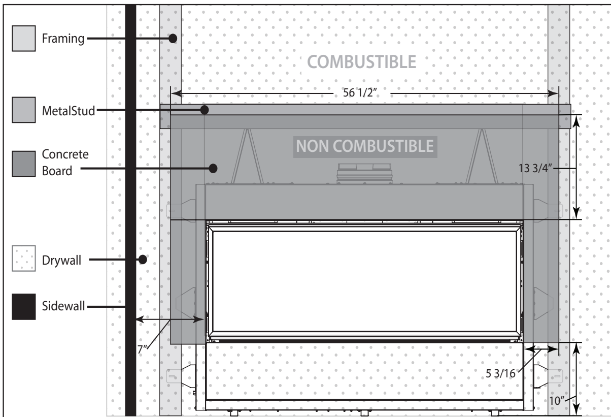
Figure 20: Finishing Non-Combustible Zones
