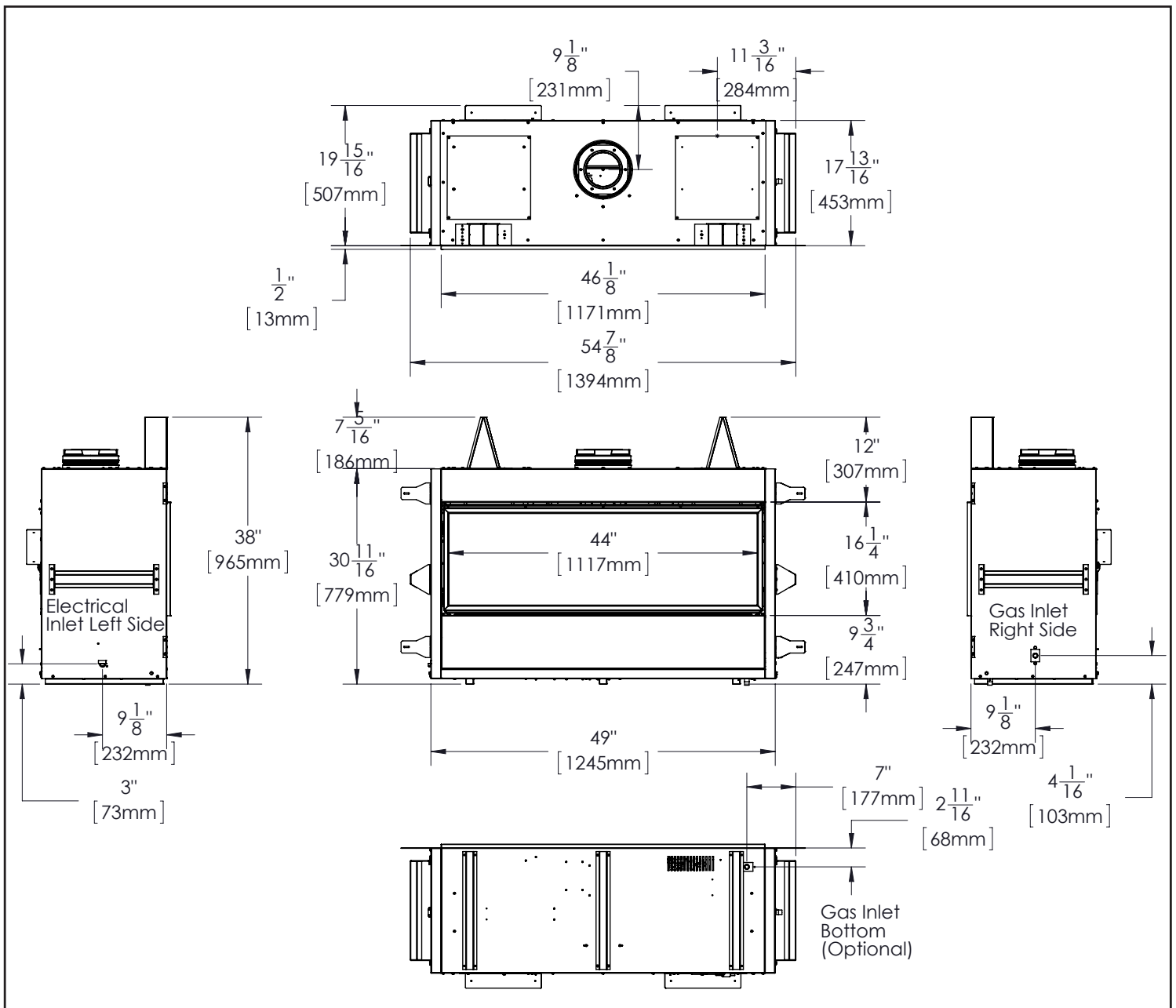
Figure 1: Unit Dimensions
